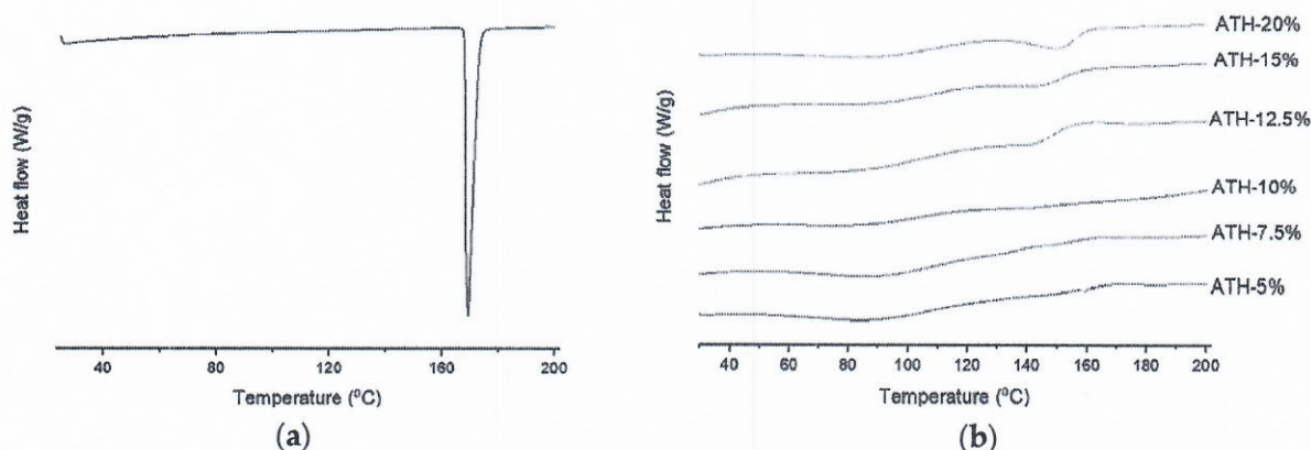
Figure 5. DSC (differential scanning calorimetry) thermograms of: (a) pure ATH prior to printing, and (b) the DLP 3D-printed tablets with different amounts of ATH.
