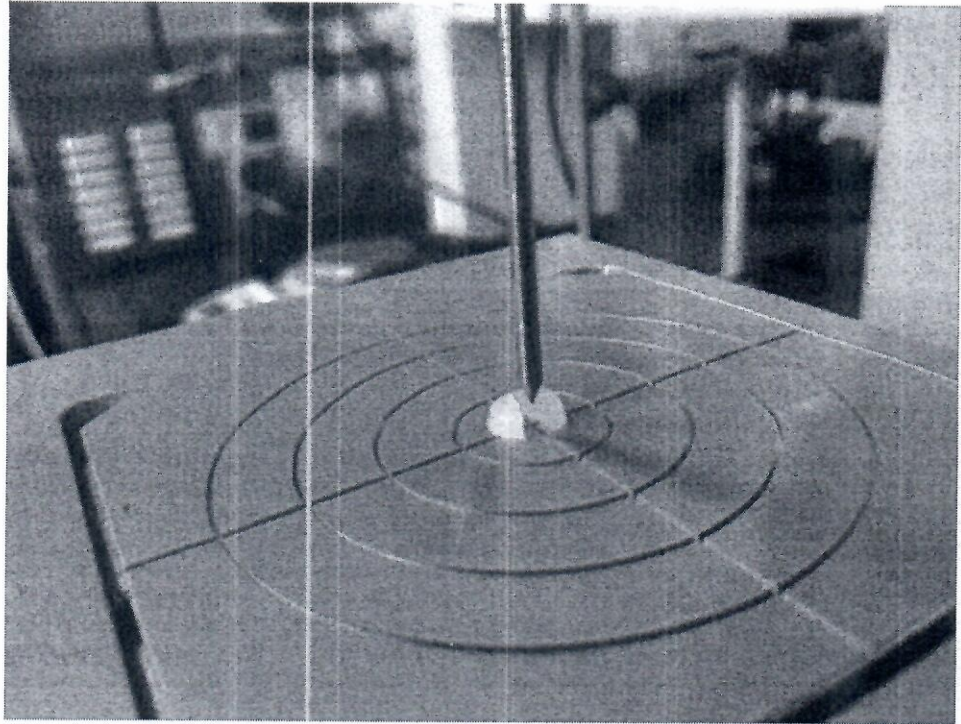
Figure 3. Determination of mechanical properties of the tablets on EZ-LX Compact Table-Top Testing Machine.
