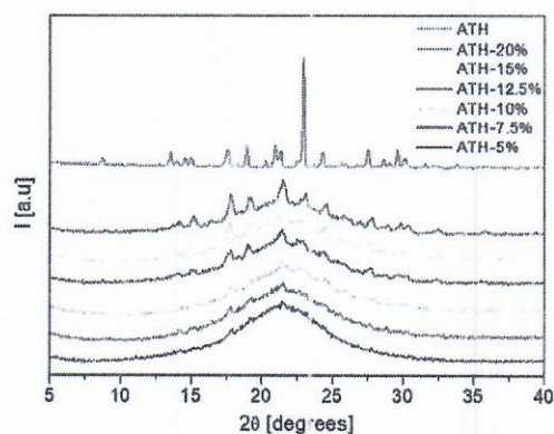
Figure 6. The X-ray powder diffraction (XRPD) patterns of raw unprocessed ATH and fabricated tablets.
