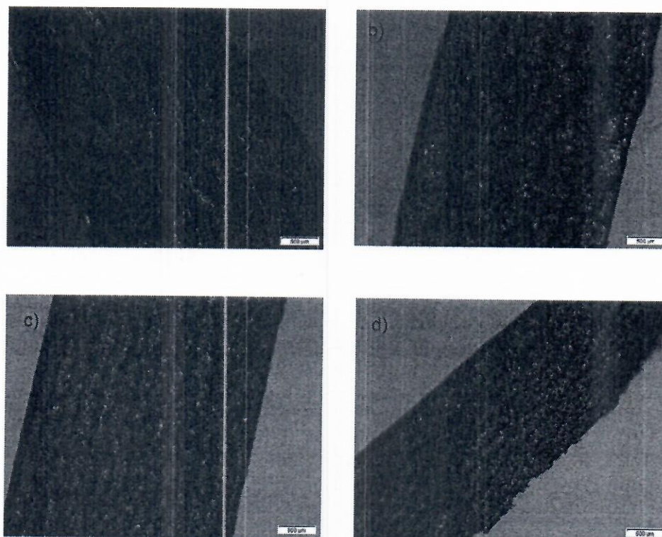
Figure 7. Cross section of tablets before dissolution testing containing: (a) 5%; (b) 10%; (c) 15%; (d) 20% of ATH.
