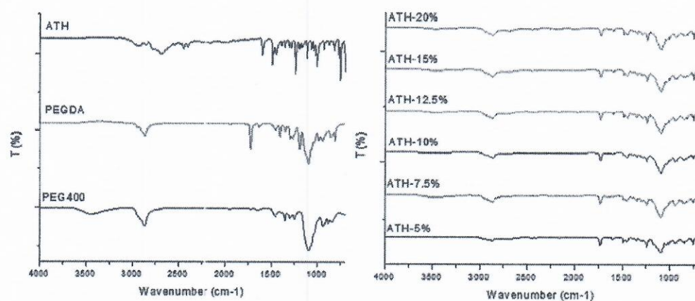
Figure 9. Fourier-transform infrared (FTIR) spectra of substances (left) and fabricated tablets (right).
